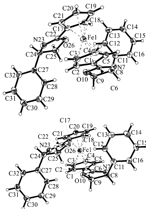
Figure 3. The molecular structure and labeling scheme of 1,1'-bis[( R )-4-phenyloxazolin-2-yl]ferrocene ( 13b ; top) and 1,1'-bis[( S )-4-phenyloxazolin-2-yl]ferrocene ( 14b ; bottom) with displacement ellipsoids drawn at the 50% probability level.
