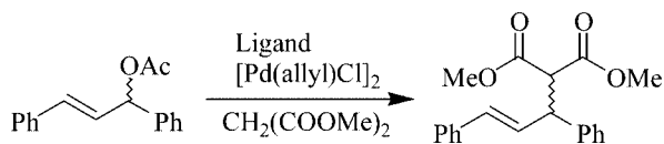
Scheme 2. General scheme for the palladium-catalyzed allylic alkylation.
