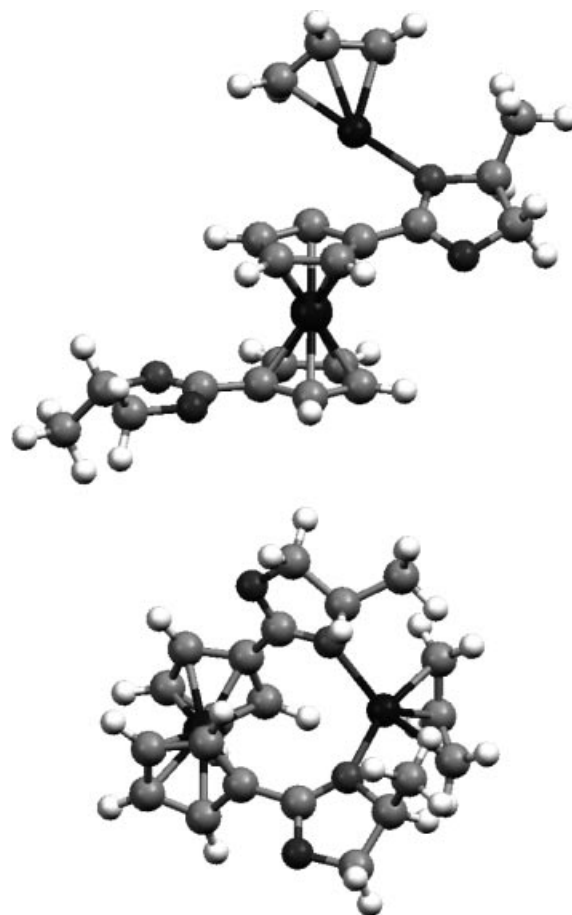
Figure 5. Equilibrium structures of complexes 1c (top) and 1d (bottom).
