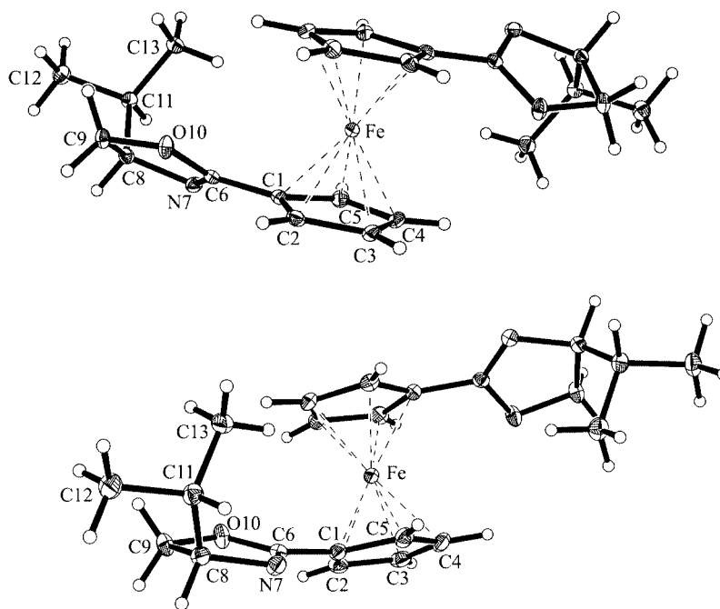
Figure 1. The molecular structure and labeling scheme of 1,1'-bis[( R )-4-isopropylloxazolin-2-yl]ferrocene ( 6b ; top) and 1,1'-bis[( S )-4-isopropylloxazolin-2-yl]ferrocene ( 7b ; bottom) with displacement ellipsoids drawn at the 50% probability level.
