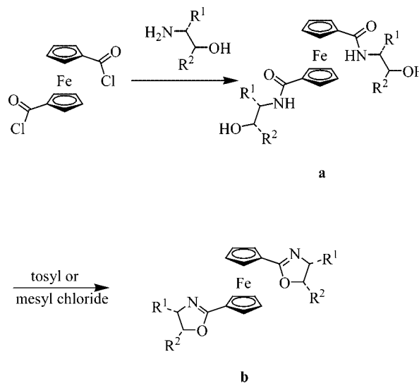
Scheme 1. General scheme for the synthesis of the 1,1'-bis(oxazolin-2-yl)ferrocenes.
