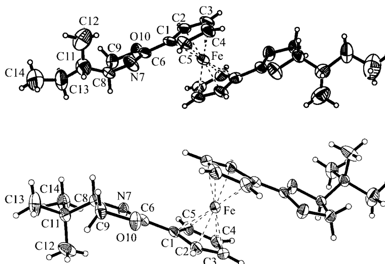
Figure 2. The molecular structure and labeling scheme of 1,1'-bis[( S )-4- sec -butyloxazolin-2-yl]ferrocene ( 11b ; top) and 1,1'-bis[( S )-4- tert -butyloxazolin-2-yl]ferrocene ( 12b ; bottom) with displacement ellipsoids drawn at the 50% probability level.
