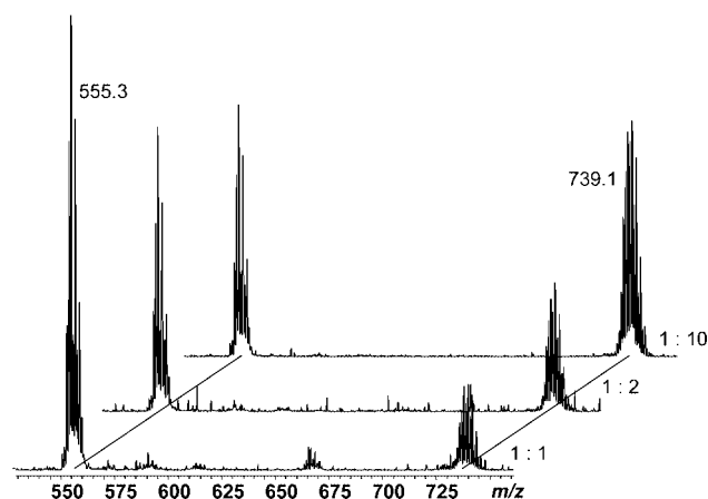
Figure 4. Mass spectrometric investigation of the coordination behavior of 1,1'-bis[( S )-4-isopropoxyloxazolin-2-yl]ferrocene ( 7b ) toward [\text{Pd}(\text{allyl})\text{Cl}]_2 at molar ratios of 1:1, 1:2, and 1:10 (ligand/palladium), with peaks found at m/z = 555 and 739 assignable to the mono- and bis-palladium complexes, respectively.
